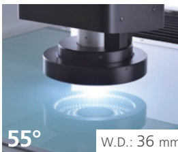
• LED outer ring light at 55 degree position
