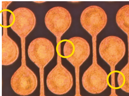
Micro wiring patterns (Type2 head, optical magnification 15×)
