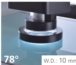
• LED outer ring light at 78 degree position
